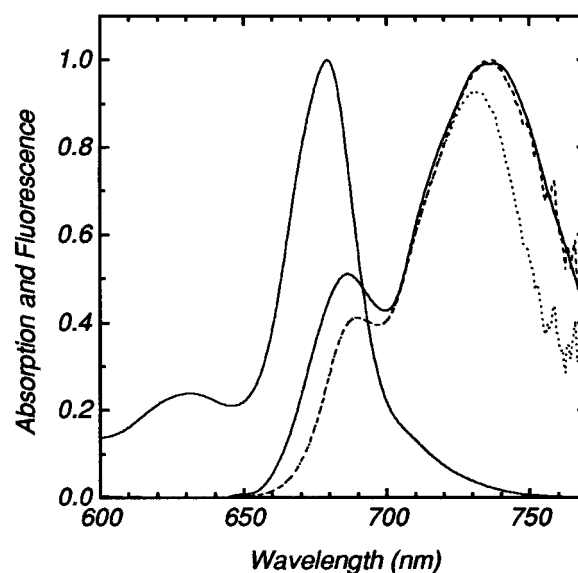
FIGURE 6 Comparison between the calculated (dashed line) and the measured steady-state fluorescence spectra (solid line) for photosystem I trimers of Spirulina at room temperature. The emission spectrum was calculated from the absorption spectrum, also shown in the figure, by the Stepanov equation (see text). The dotted-line fluorescence spectrum was calculated from the absorption spectrum in the same way but after subtraction of the minor, 743-nm absorption sub-band.
