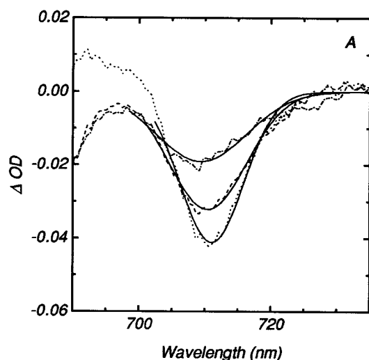
FIGURE 3 Photobleaching hole in the long wavelength absorption tail of Spirulina trimers at selected temperatures. Spectra were calculated as the photobleached samples minus control after normalization as shown in Fig. 2. Experimental difference spectra are shown by broken lines and the Gaussian approximations by solid lines for 280 K, 180 K, and 100 K.
